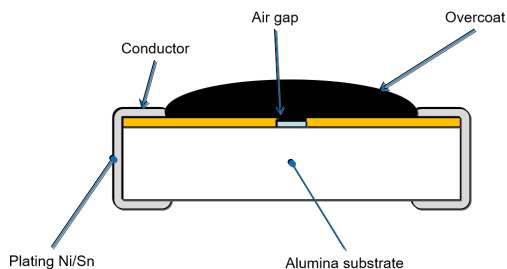
TFE series structure
